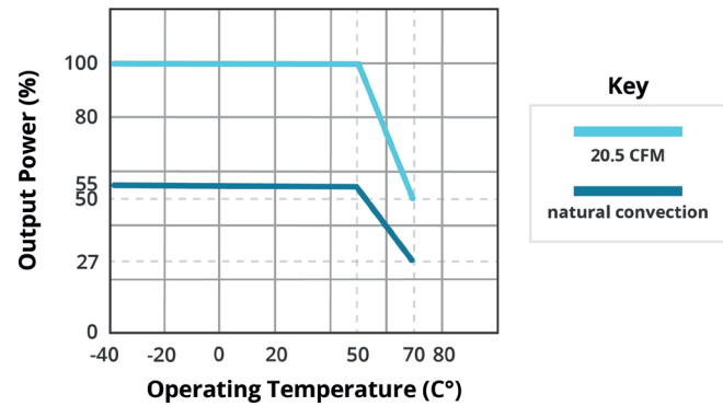
TEMPERATURE DERATING CURVE VMS-350C-15 (full load 325W with 20.5 CFM)
