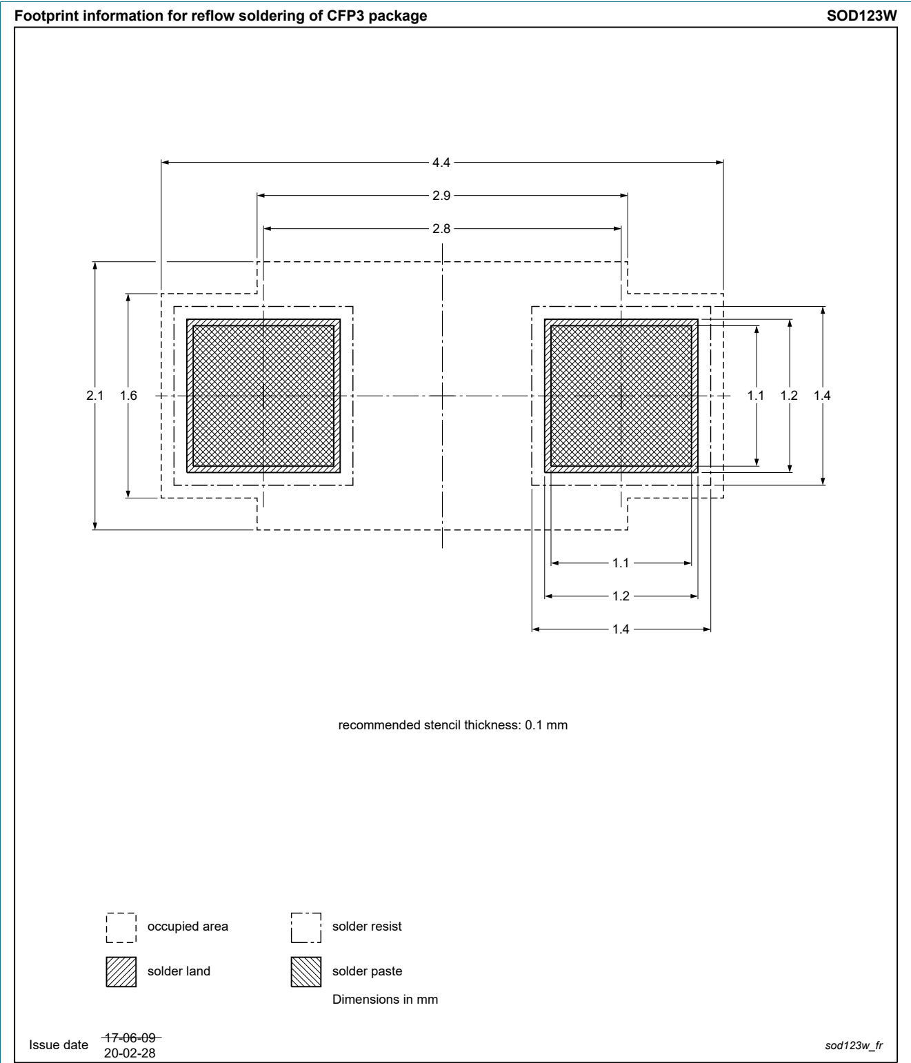
Fig. 19. Reflow soldering footprint for CFP3 (SOD123W)
