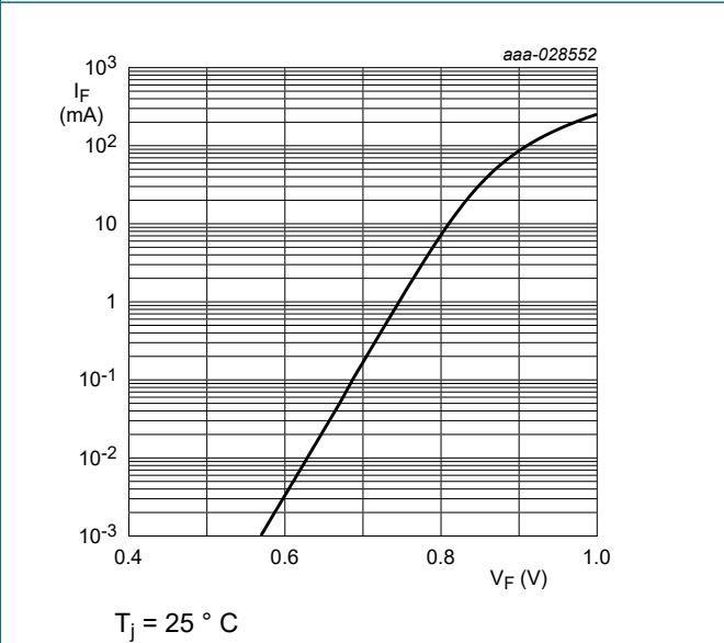
Fig. 3. Forward current as a function of forward voltage; typical values (MM5Z7V5T5G)
