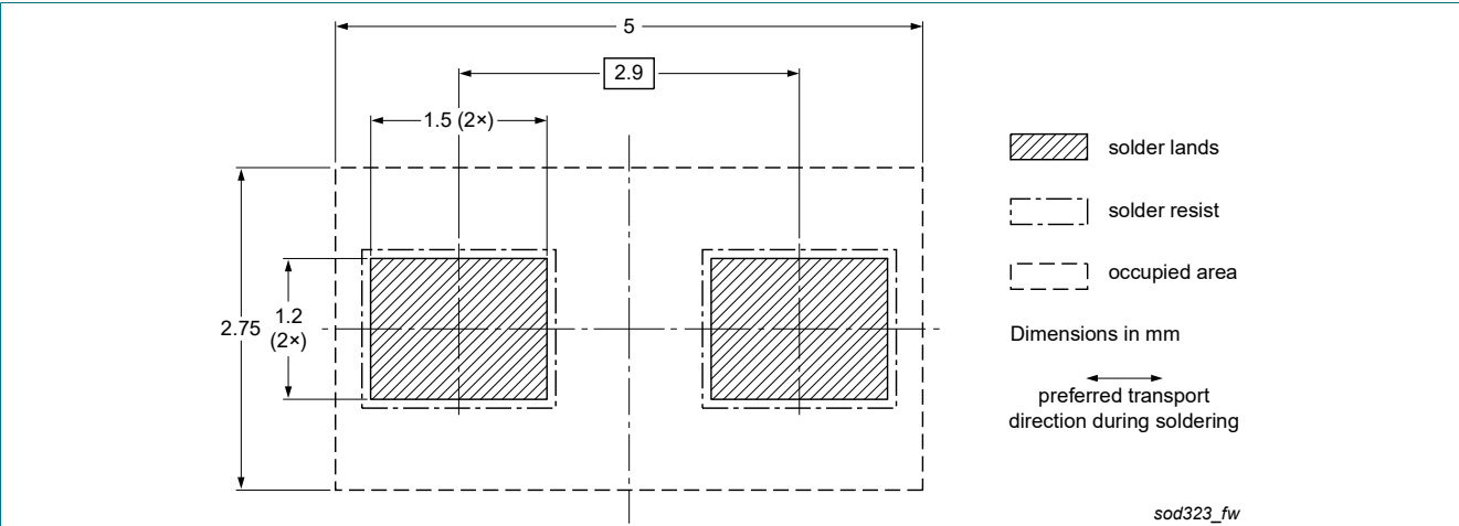
Fig. 13. Wave soldering footprint SOD323 (SC-76)
