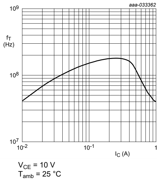
Fig. 10. Transition frequency as a function of collector current; typical values
