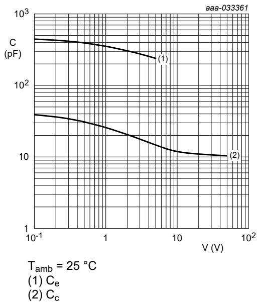
Fig. 9. Input/output capacitance as a function of input/output voltage
