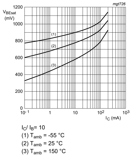
Fig. 7. BC846AQC-Q: Base-emitter saturation voltage as a function of collector current; typical values
