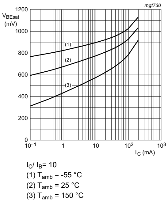
Fig. 11. BC846BQC-Q: Base-emitter saturation voltage as a function of collector current; typical values
