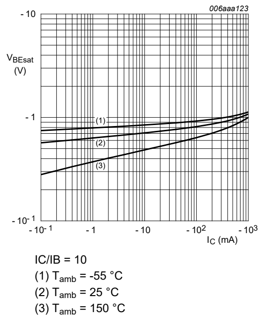
Fig. 10. BC807-25QC-Q: Base-emitter saturation voltage as a function of collector current; typical values
