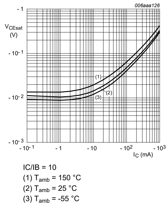
Fig. 11. BC807-25QC-Q: Collector-emitter saturation voltage as a function of collector current; typical values
