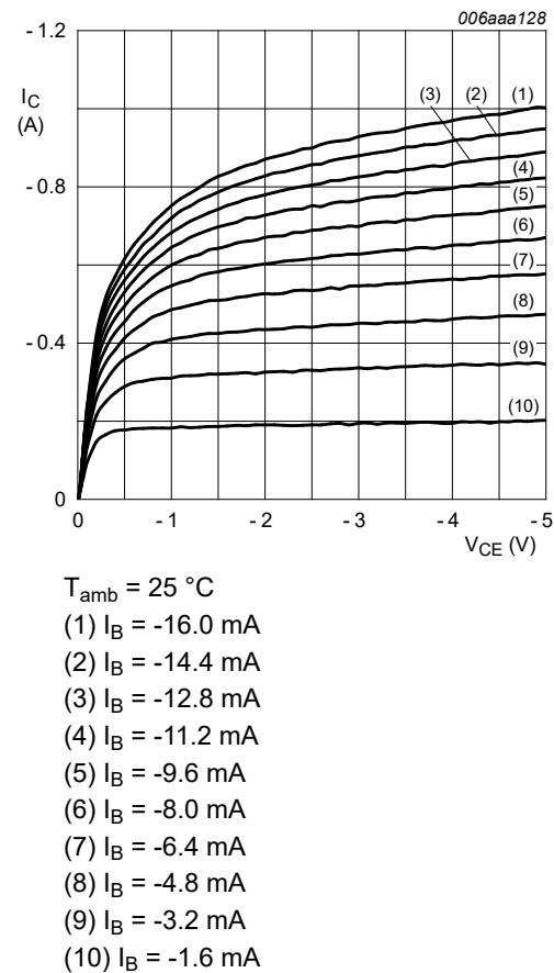
Fig. 5. BC807-16QC-Q: Collector current as a function of collector-emitter voltage; typical values
