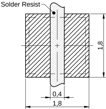
No vias and traces in restricted area. Scale - 15:1
