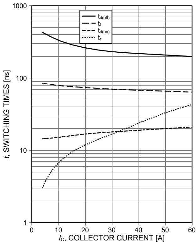
Figure 7. Typical switching times as a function of collector current (inductive load, T vj =175°C, V CE =400V, V GE =15/0V, r G =12Ω, Dynamic test circuit in Figure E)
