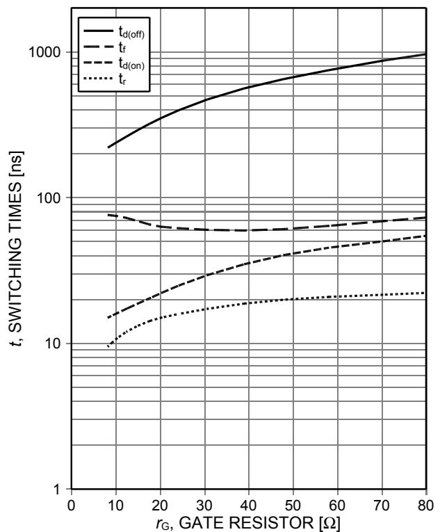
Figure 8. Typical switching times as a function of gate resistor (inductive load, T vj =175°C, V CE =400V, V GE =15/0V, I C =20A, Dynamic test circuit in Figure E)
