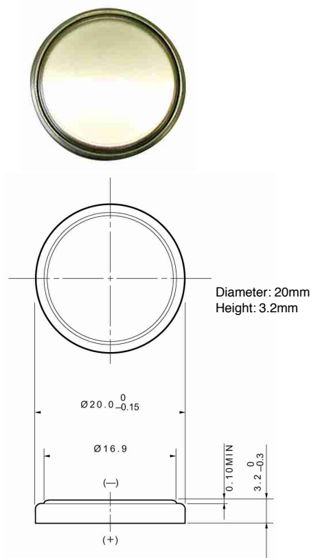
Dimension Drawing
