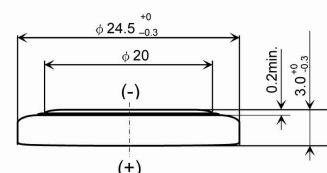
Dimension Drawing
