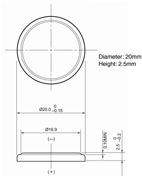
Dimension Drawing
