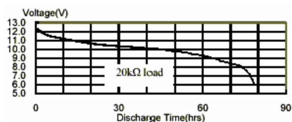
Typical Discharge characteristics at 20 \pm 2^\circ\text{C}
