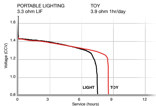
Application Tests (23±2°C)
