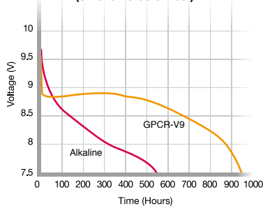
ANSI 10K ohm background 24hr/day 620 ohm 1 sec/hr to 5.4V at 23°C (Smoke Detector Test)
