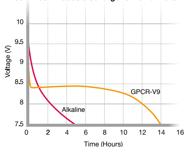
50mA continuous discharge to 7.5V at 23°C
