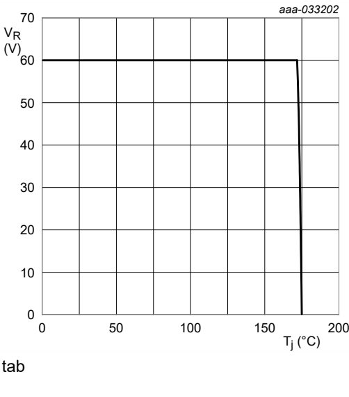
Fig. 13. Derated maximum reverse voltage as a function of junction temperature; typical values
