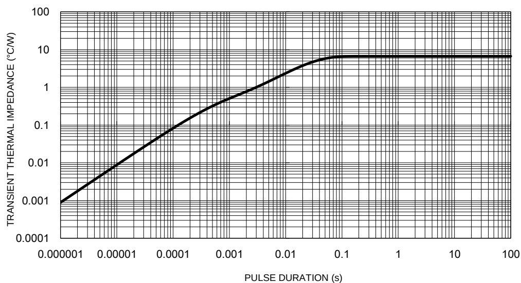
Fig.5 Typical Transient Thermal Impedance
