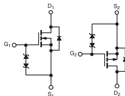
N-Channel MOSFET
