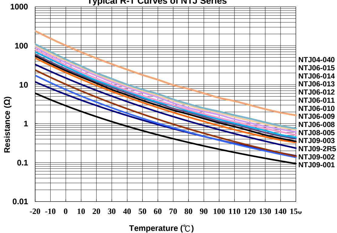
Typical R-T Curves of NTJ Series
