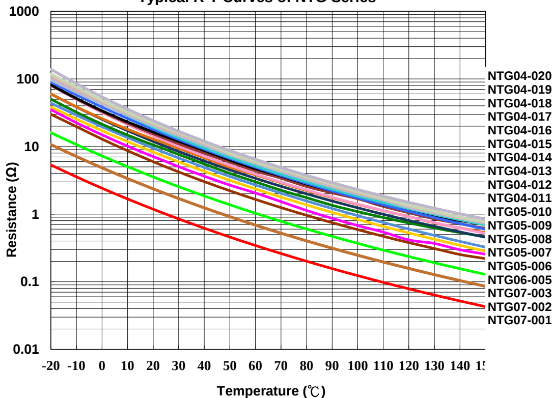
Typical R-T Curves of NTG Series
