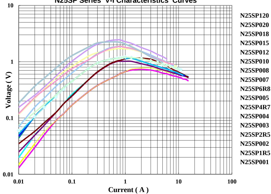
N25SP Series V-I Characteristics Curves
