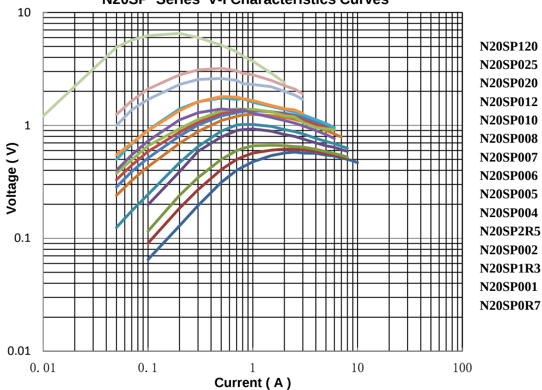
N20SP Series V-I Characteristics Curves
