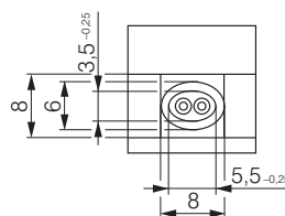
Leads end B
