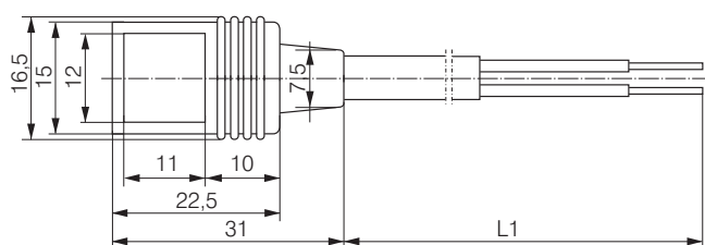
Connector cable
