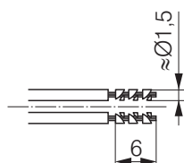
Core crimp sleeve
