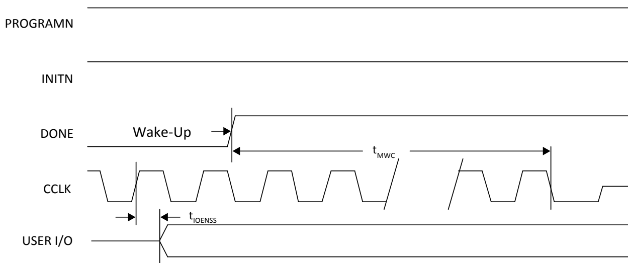
Figure 3.21. Wake-Up Timing
