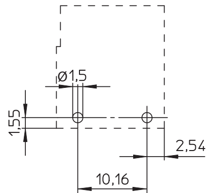
PCB LAYOUT - COMPONENT VIEW
