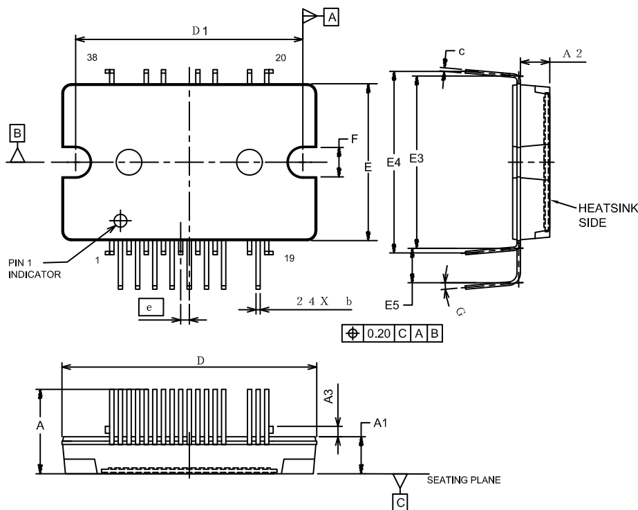
DIP38 29.60x18.20 EP-5 CASE 181AE ISSUE O
