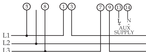
For 3 Phase 3 Wire Unbalanced Load
