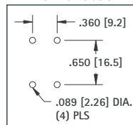
Mounting Detail For Two Holders
