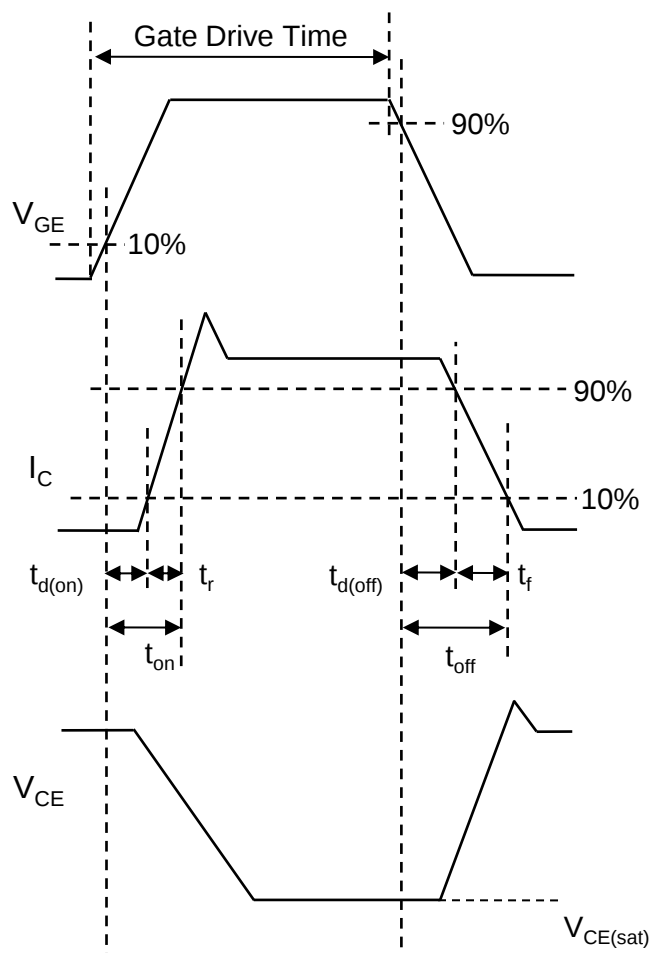
Fig.19 Inductive Load Waveform
