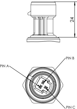
PACKARD METRI-PACK 150 IP67
