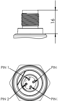
M12x1 4-POLE IP67
