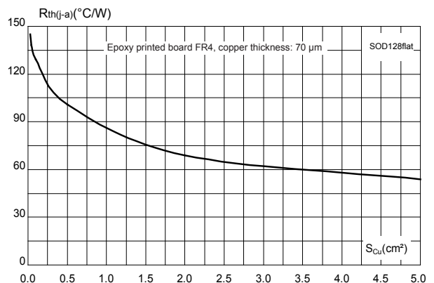
Figure 6. Thermal resistance junction to ambient versus copper surface under each lead (typical values, epoxy printed board FR4, e_{Cu} = 70 \mu m )
