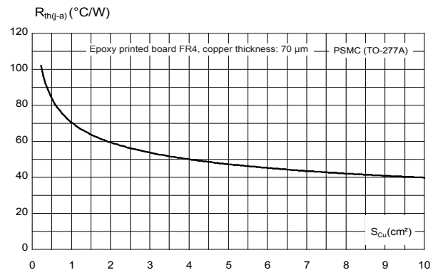
Figure 6. Thermal resistance junction to ambient versus copper surface under tab (typical values, epoxy printed board FR4, e_{Cu} = 70 \mu m )
