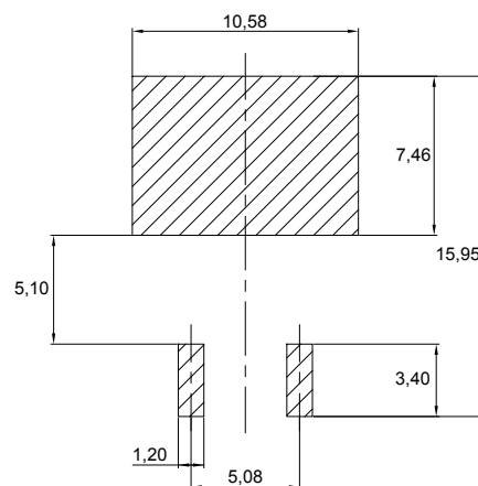
Figure 10. D 2 PAK high voltage footprint in mm
