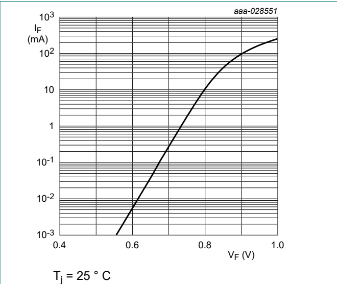
Fig. 2. Forward current as a function of forward voltage; typical values (SZMM5Z6V8T5G)
