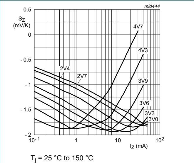
Fig. 4. Temperature coefficient as a function of working current; typical values (SZMM5Z2V4T5G to 4V7T5G)
