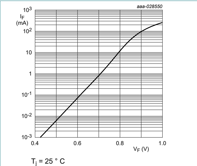
Fig. 1. Forward current as a function of forward voltage; typical values (SZMM5Z2V4T5G)
