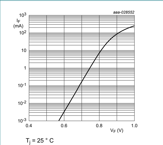
Fig. 3. Forward current as a function of forward voltage; typical values (SZMM5Z7V5T5G)
