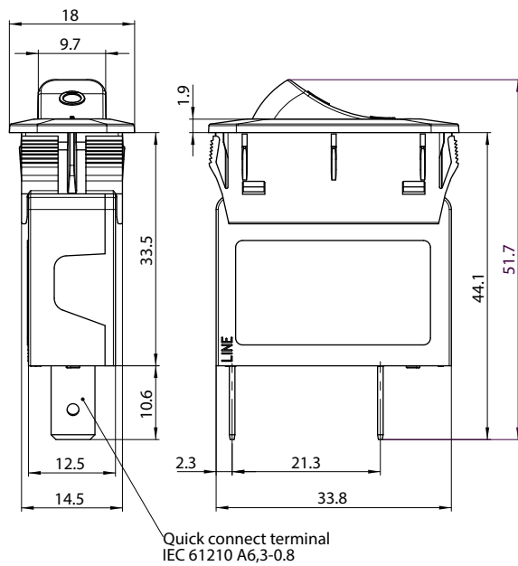
1-pole
