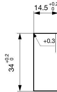
Panel 1.0 – 3.5 mm
