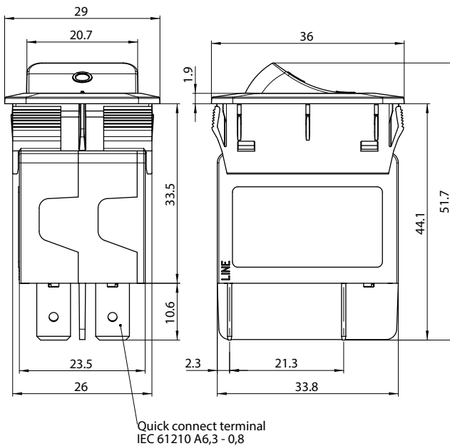
2-pole
