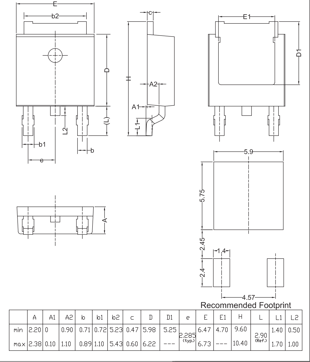
Plastic single-ended surface-mounted package (DPAK); 3 leads (one lead cropped) TO252
