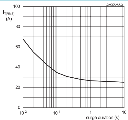
Fig. 2. RMS on-state current as a function of surge duration; maximum values f = 50\text{ Hz} ; T_{\text{mb}} = 121^\circ\text{C}
