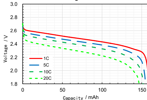
Discharge characteristics
