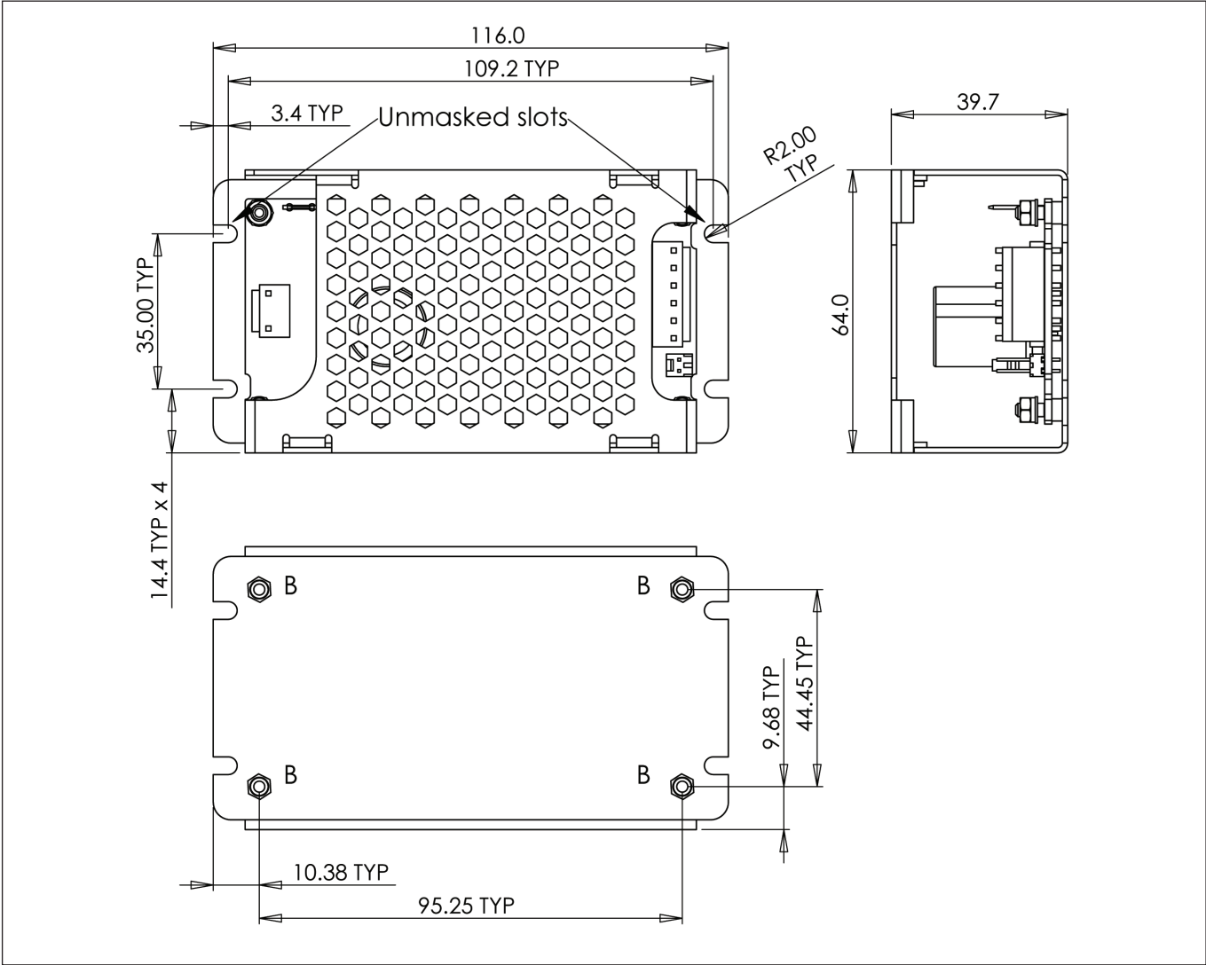
Outline Drawing CUS150M/A (U Channel with Cover) Option
