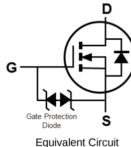
Equivalent Circuit
