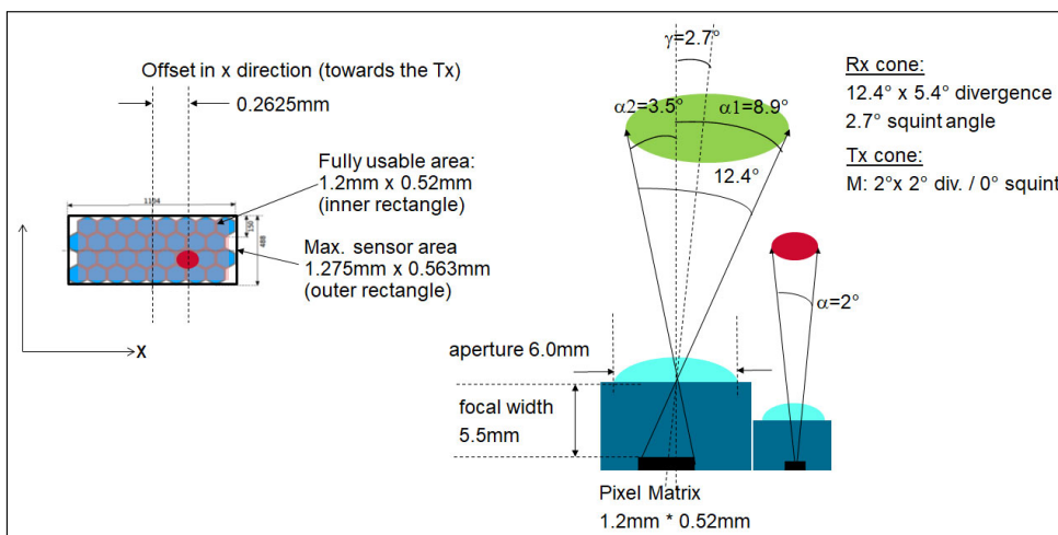
Figure 6: Field-of-View (FoV) Description of the Sensor
