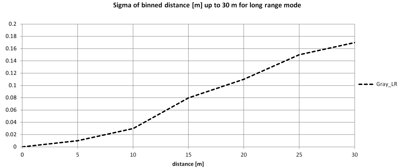
Figure 9: Standard Deviation Distance Measurement from 0 to 30m with frame rate of 25Hz
