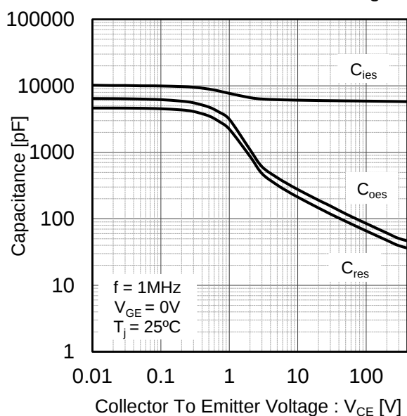
Fig.11 Typical Capacitance vs. Collector to Emitter Voltage
