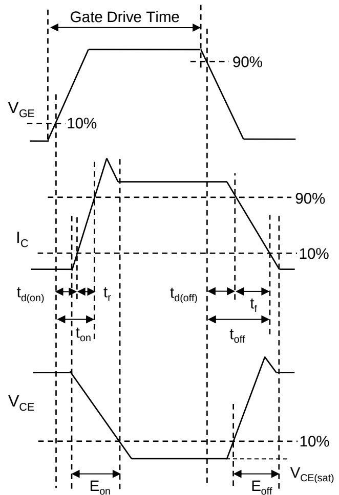
Fig.23 Inductive Load Waveform
