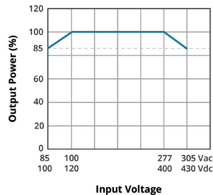
INPUT VOLTAGE DERATING CURVE (25°C)
