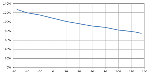
Temperature Derating Curve
