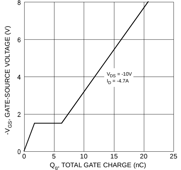
Figure 10 Gate-Charge Characteristics
