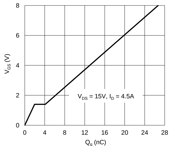
Figure 12. Gate Charge
