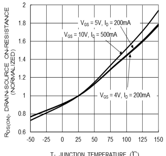
Figure 6. On-Resistance Variation with Junction Temperature
