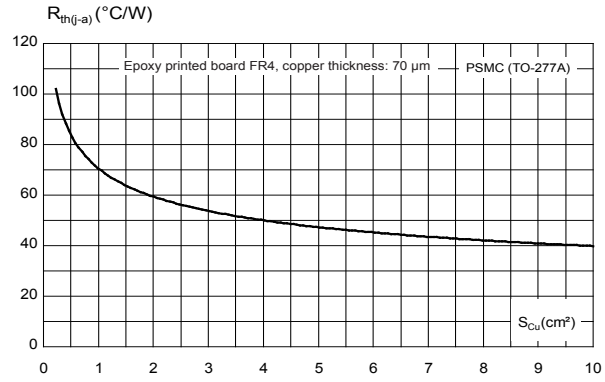
Figure 7. Thermal resistance junction to ambient versus copper surface under tab (typical values, epoxy printed board FR4, e_{Cu} = 70 \mu\text{m} ) (PSMC (TO-277A))
