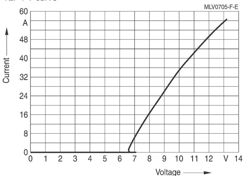
TLP I-V curve
