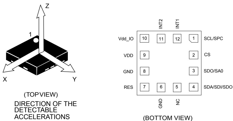
Figure 2. Pin connections
