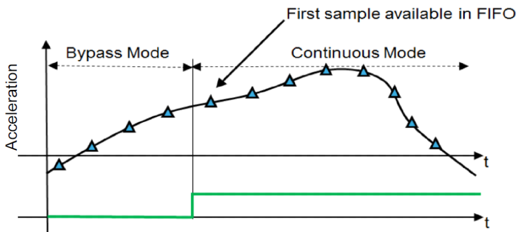
Figure 11. Trigger event to FIFO for Bypass-to-Continuous mode
