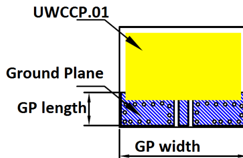
Figure 3 Evaluation Board
