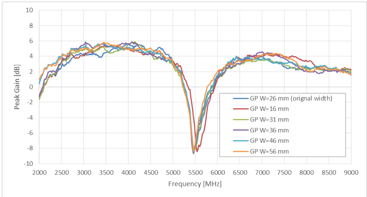
Figure 9 Peak gain for ground plane width variation
